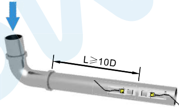
Straight length of upstream piping
